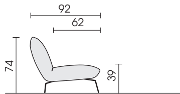
Side view (type 130)
