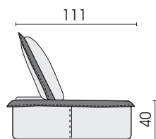
Side view, seating element, low (with backrest)
