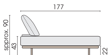
Front view (type P230/230/609)
