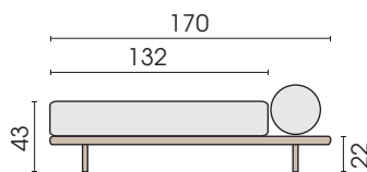
Front view (type P230/130/644)
