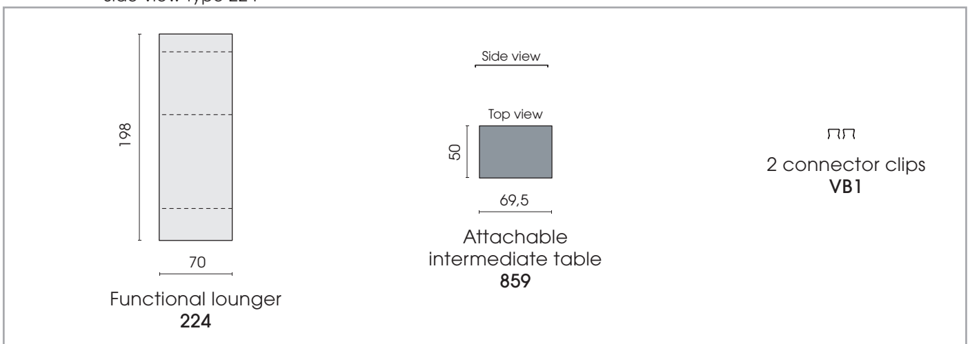
Side view type 224
